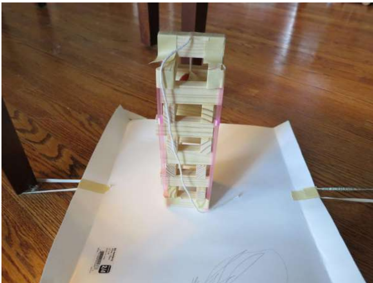
Straw re-enforced tower with a pendulum inside.
